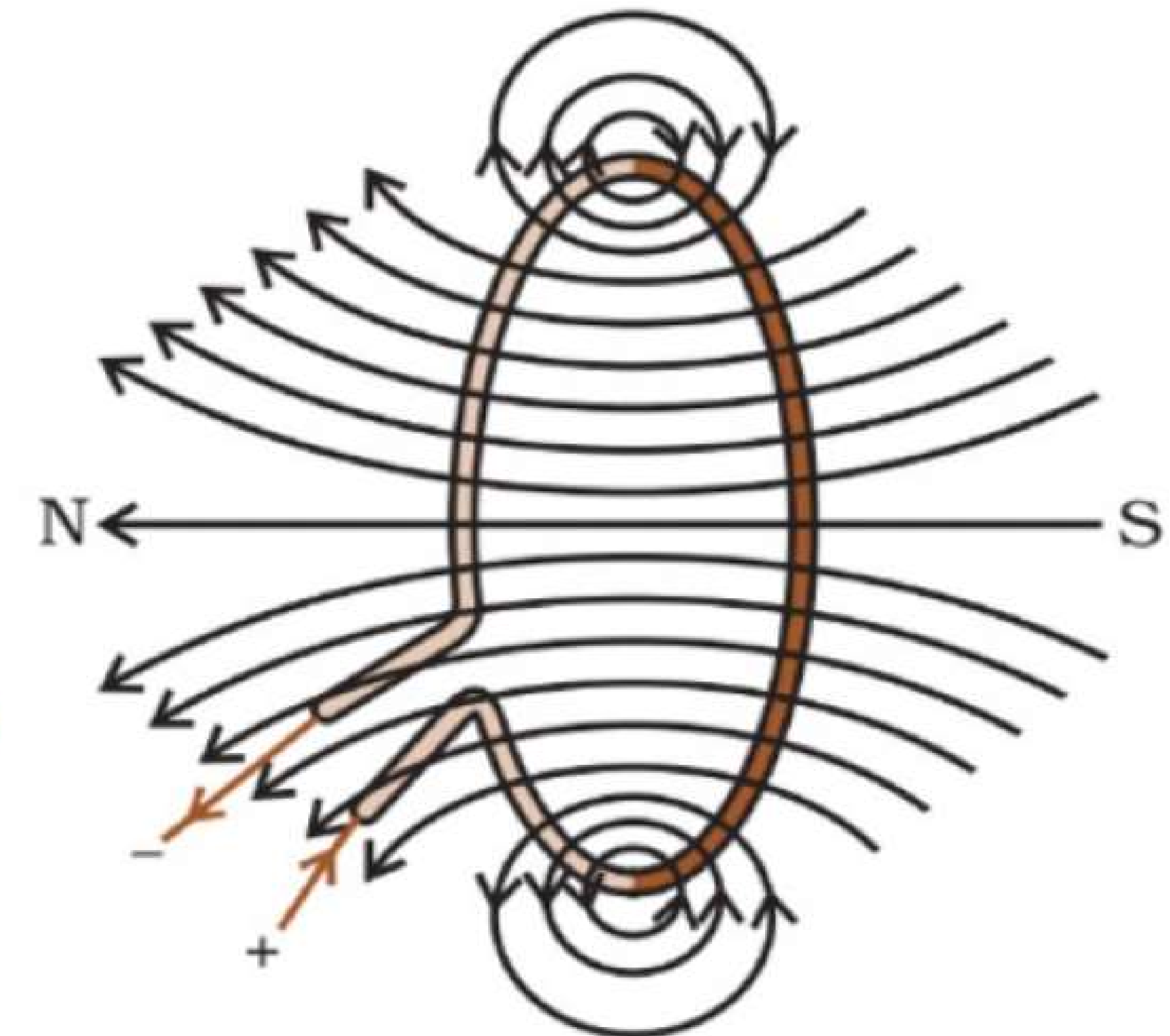
Magnetic field lines produced by a current-carrying circular loop
